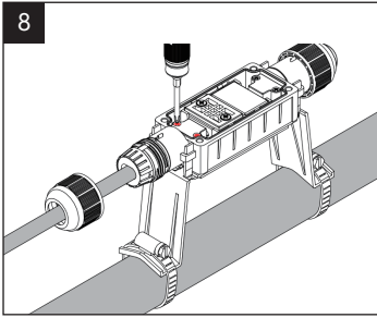
8. Tighten the two screws on the fixed cable block alternately to ensure the screws are locked.
