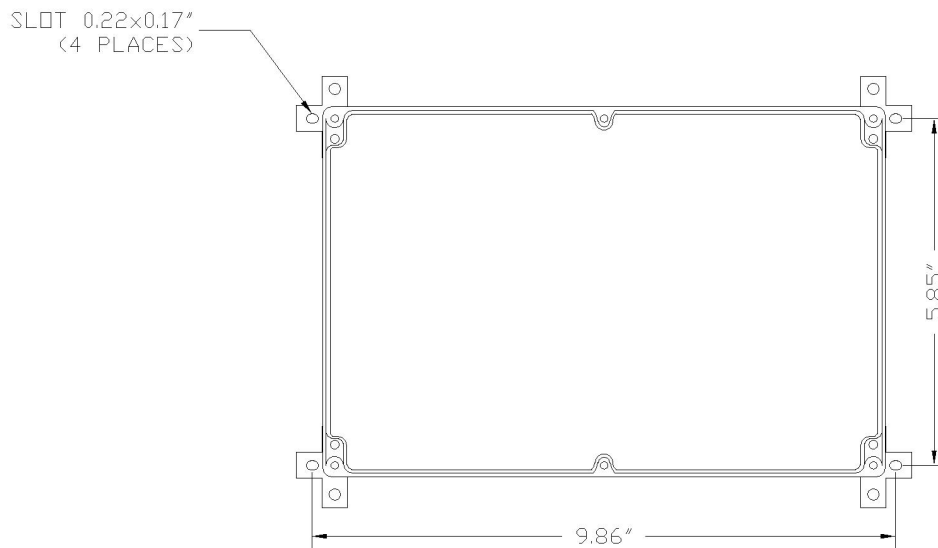
2XTC Controller Standard Mounting Feet.
